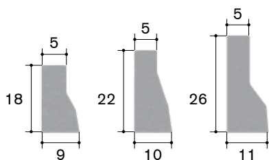
Standardelement
